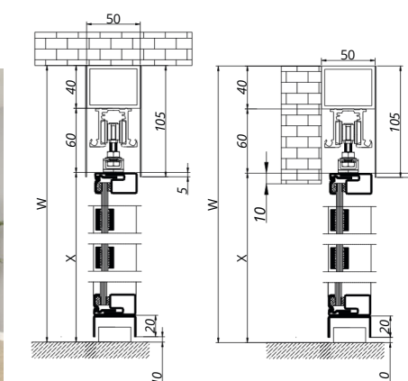
Installation to the ceiling (Standard System)
