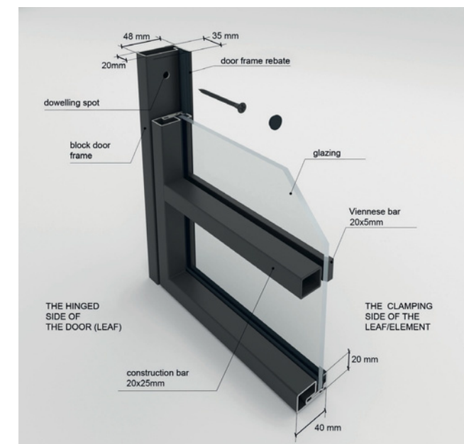
The cross-section of the frame and door leaf with a construction bar
