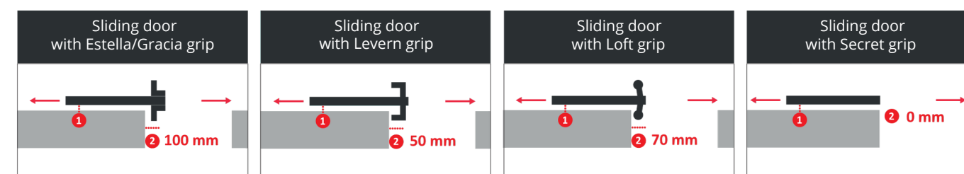
Installation to the ceiling (Standard System)
