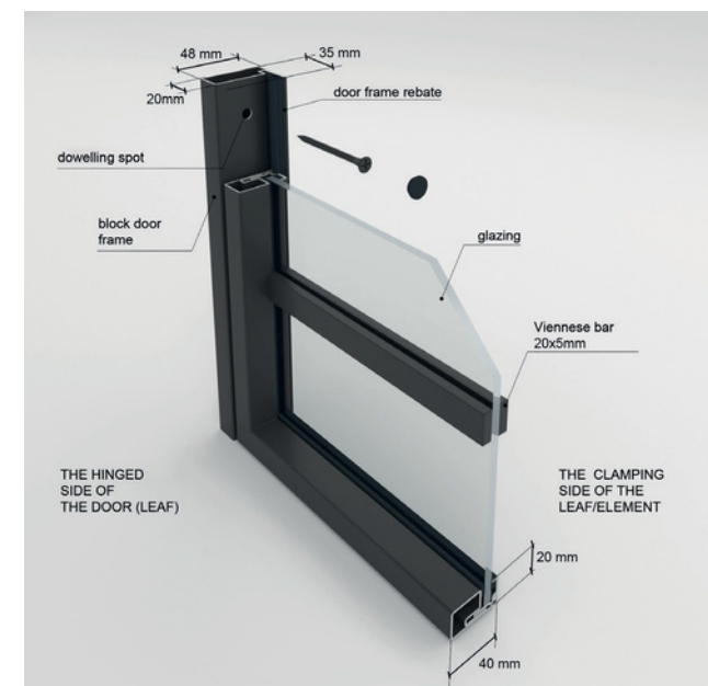
The cross-section of the frame and door leaf with a Viennese bar
