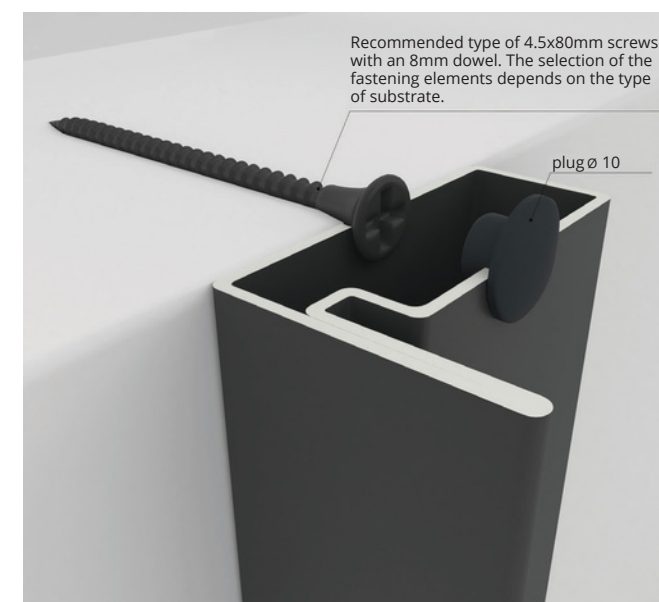
The installation of the hinged door frame
